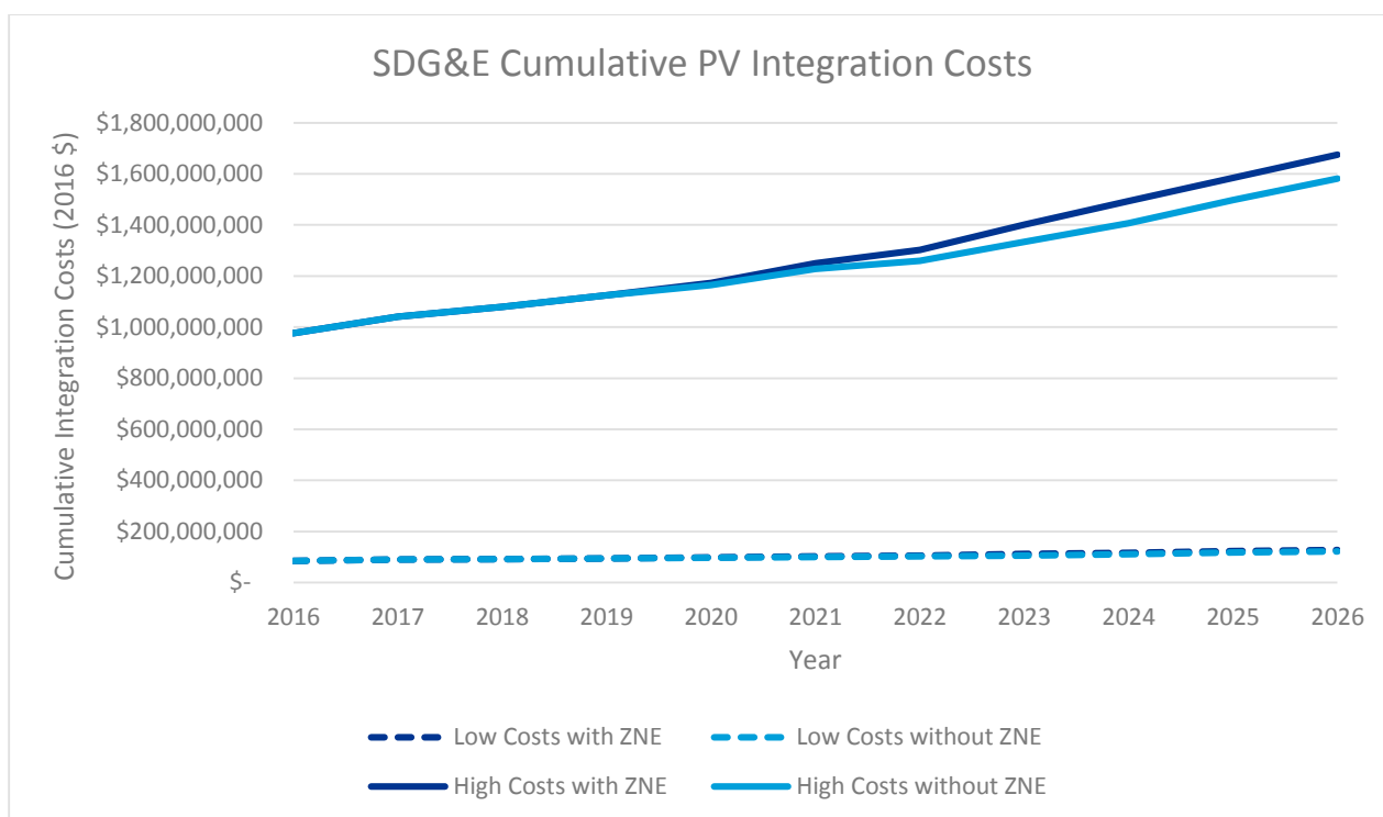
Figure 3.10: Grid integration costs for SDG&E distribution system for the 'No ZNE' and 'With ZNE' scenarios
