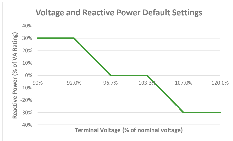
Figure 3.11: Volt/Var curve used in study
