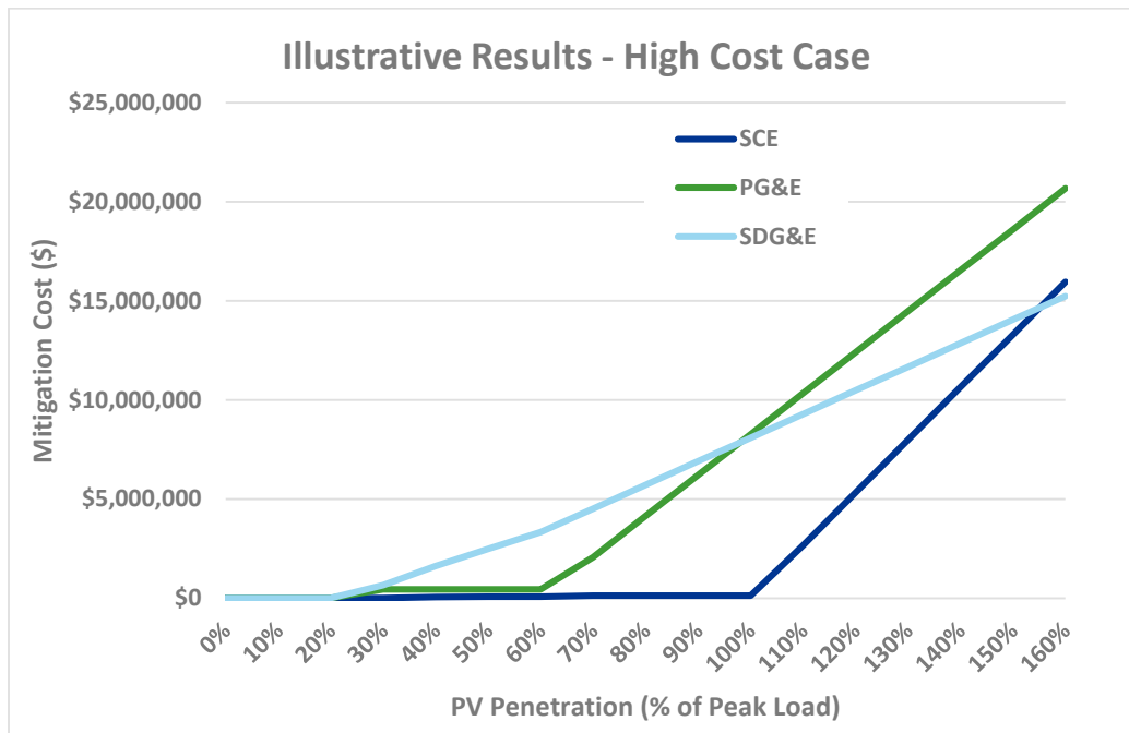
Figure 0.1: Illustrative example mitigation cost profiles for single circuits – high cost case
